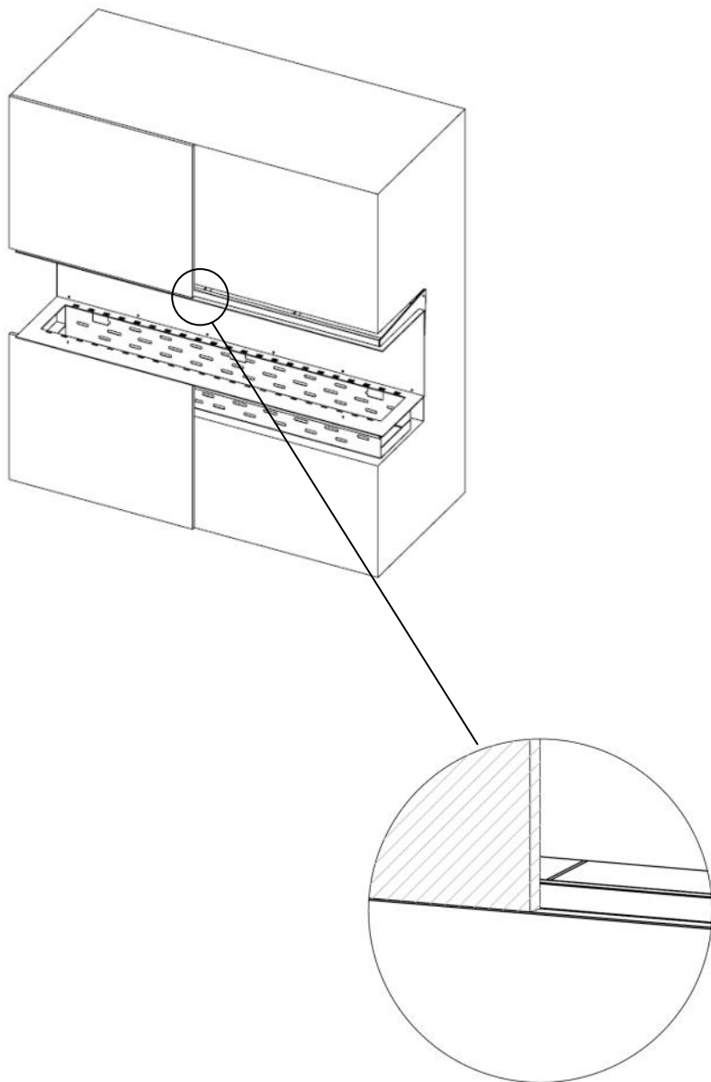
Figure 2 —Appliquer le Placoplatre
