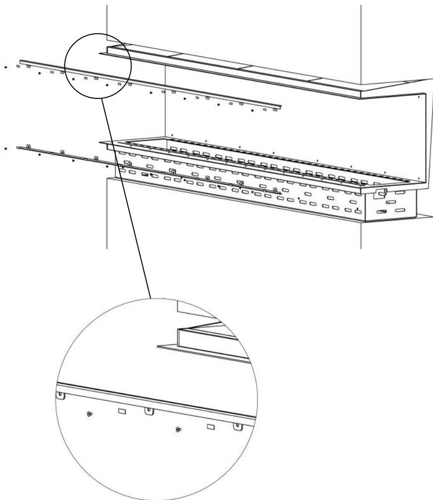
Figure 6 —Installation des supports de fixations
